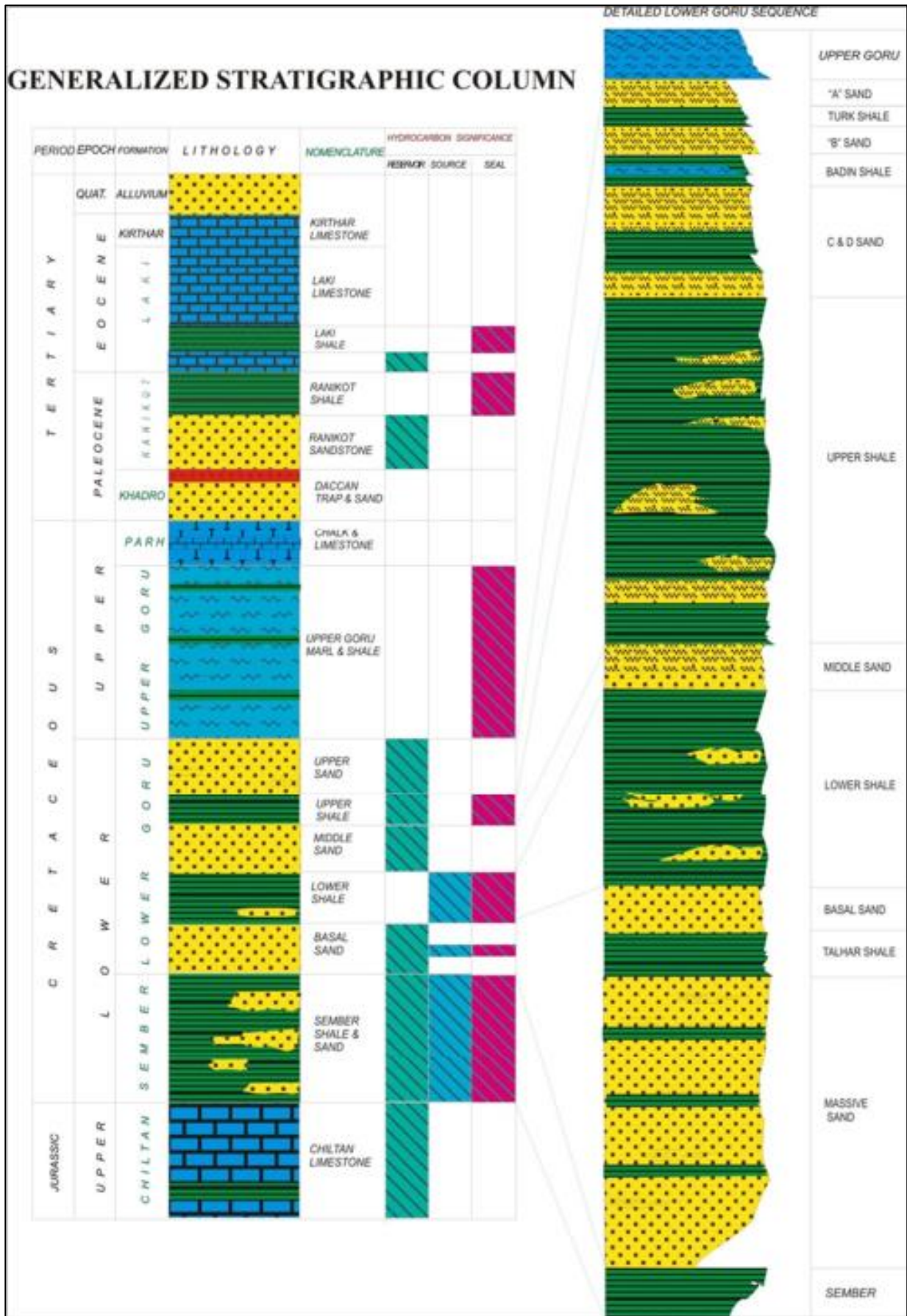
Figure 2 Generalized stratigraphic column of Lower Goru Formation
