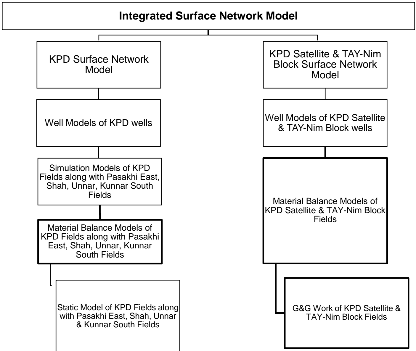
Figure 4 Study Structure
