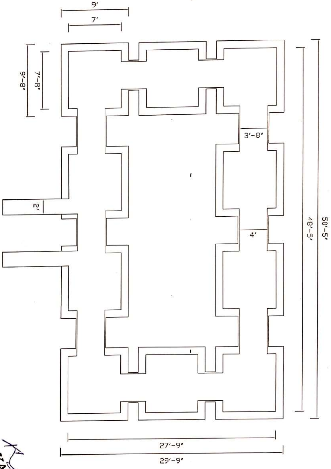
FOUNDATION PLAN
