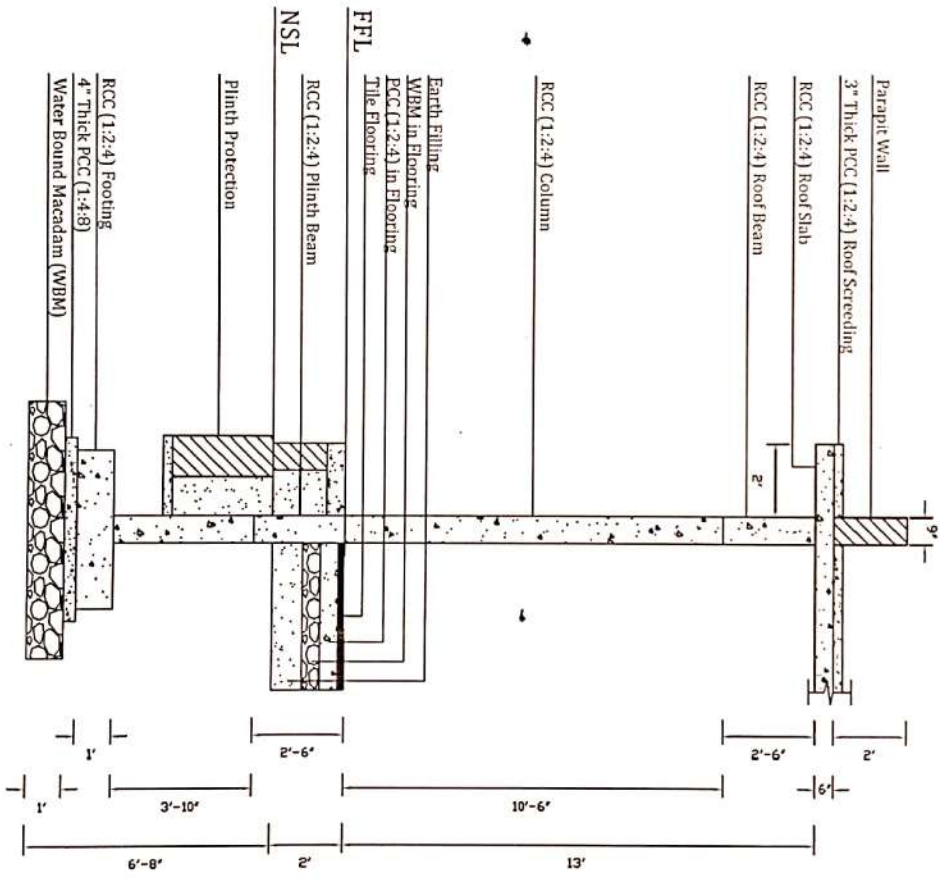
COLUMN SECTION
