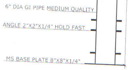
X-SECTION OF BASE PIPE GI MEDIUM QUALITY
