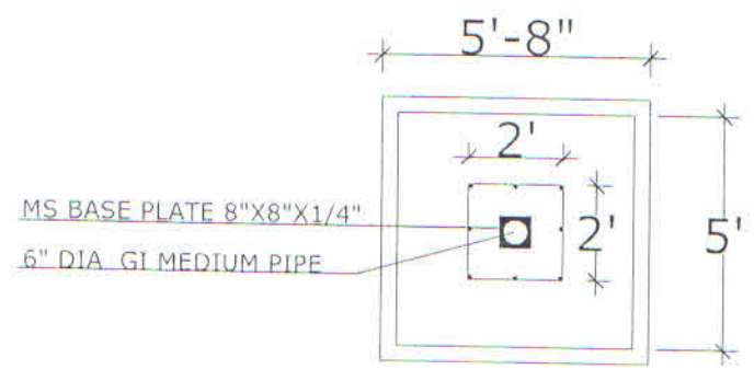
FOOTING PLAN
