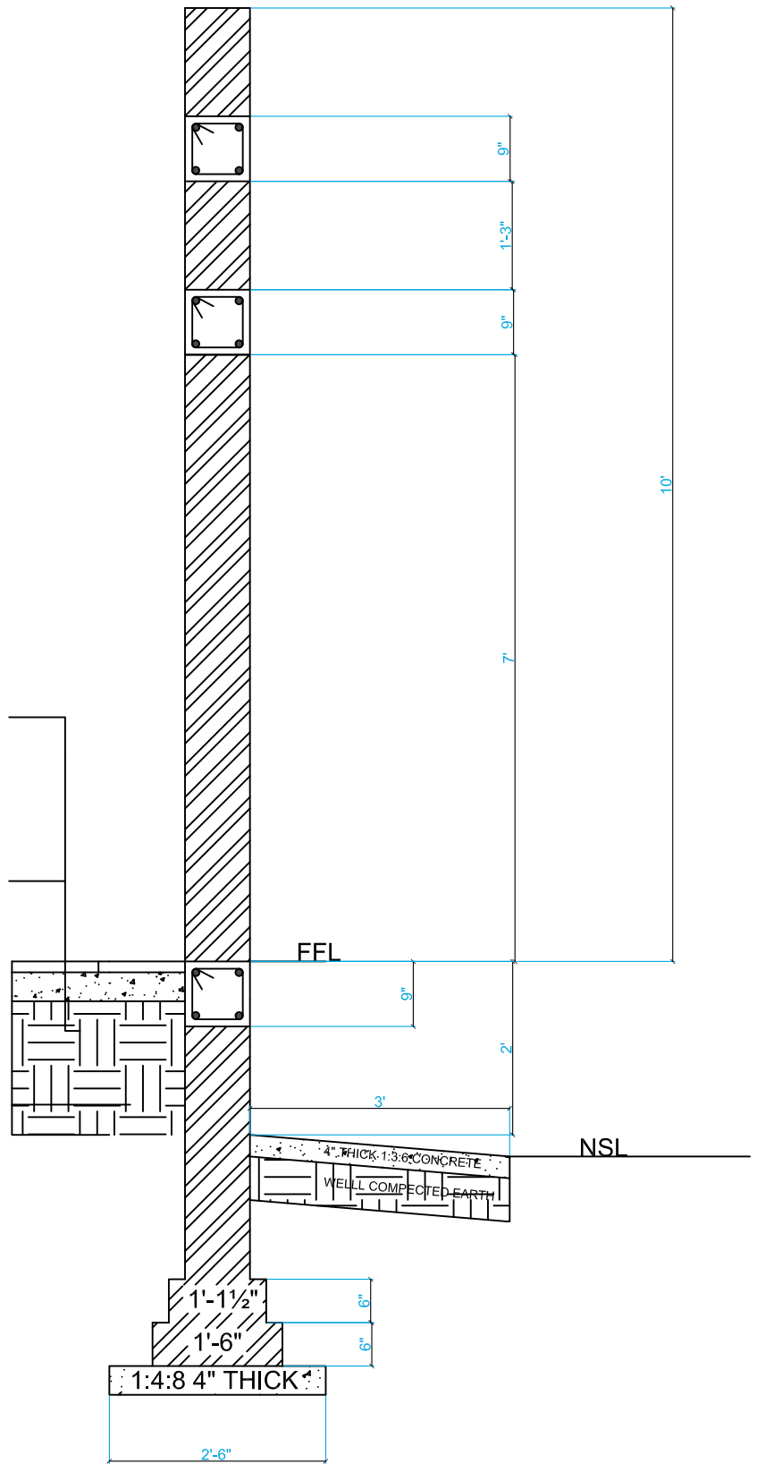
X-SEC OF 9" WALL
