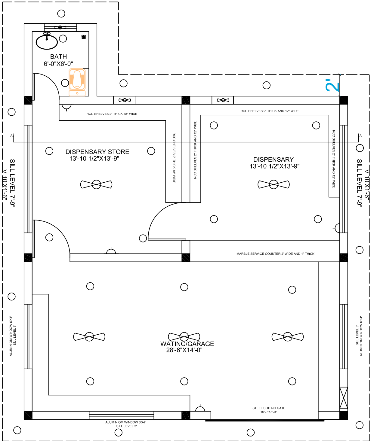
ARCHITECTURE PLAN CONSTRUCTION OF DISPENSARY AT RHC DHUMAN DISTRICT CHAKWALL
