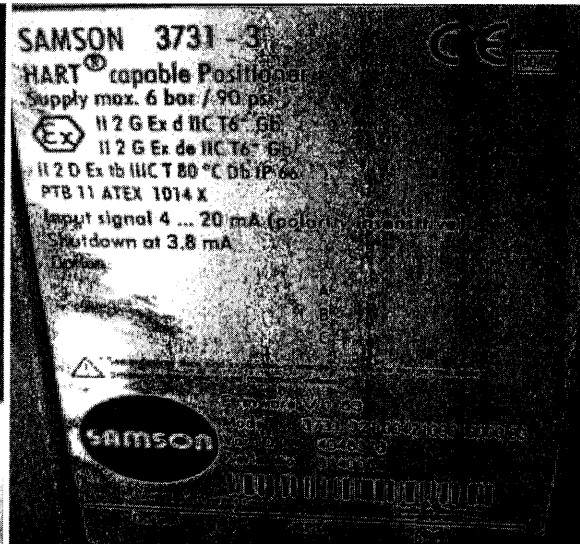
Valve Positioner 3731-321 004210001000 03
