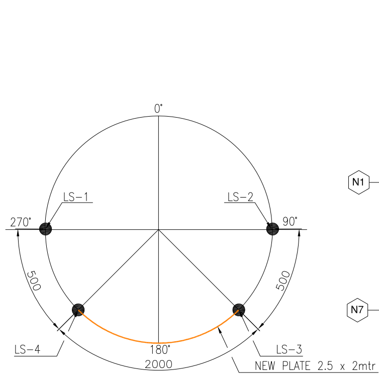
WELDING SEAM (LS) DETAIL FOR COURSE# 1 VIEW DISH-A
