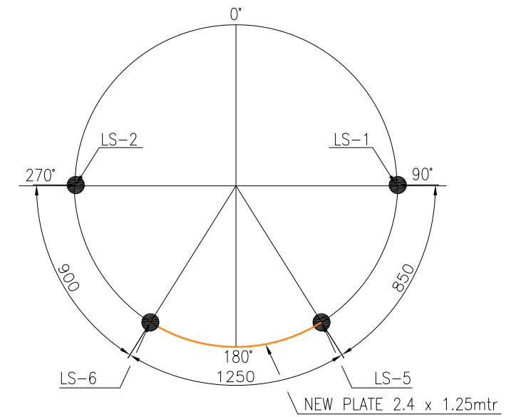
WELDING SEAM (LS) DETAIL FOR COURSE# 2 VIEW DISH-B
