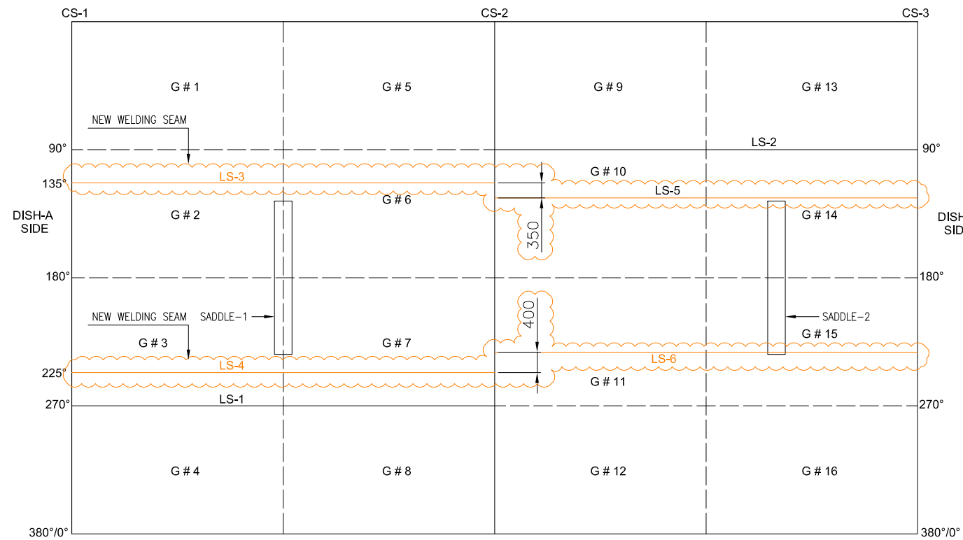
WELDING SEAM DETAIL
