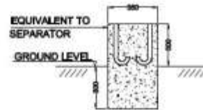
FRONT VIEW PRESSURE TRANSMITTER 2 (MOUNTING DETAILS)
