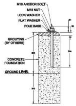
ANCHOR BOLT DETAIL FOR SOLAR POLES DETAIL A
