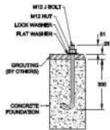
BOLT DETAIL FOR EQUIPMENT POLES DETAIL A
