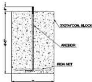
SECTION DETAIL B
