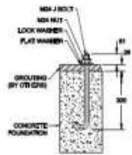
2 BOLT DETAIL FOR EQUIPMENT POLES DETAIL A
