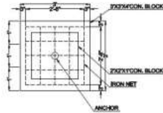
FOUNDATION PLAN DETAIL A
