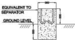
FRONT VIEW DIFFERENTIAL PRESSURE TRANSMITTER (MOUNTING DETAILS)
