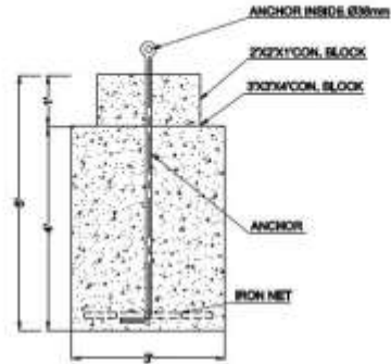
SECTION DETAIL A
