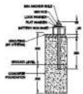
ANCHOR BOLT DETAIL FOR BATTERY BOX DETAIL C
