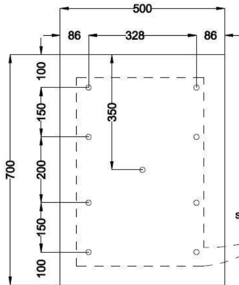
TOP VIEW ANALOG JUNCTION BOX (MOUNTING DETAILS)
