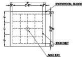
FOUNDATION PLAN DETAIL B
