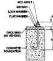
2 BOLT DETAIL FOR EQUIPMENT POLES DETAIL B
