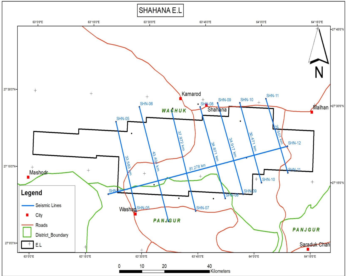
Seismic Base Map of Designed 2D Seismic acquisition program
