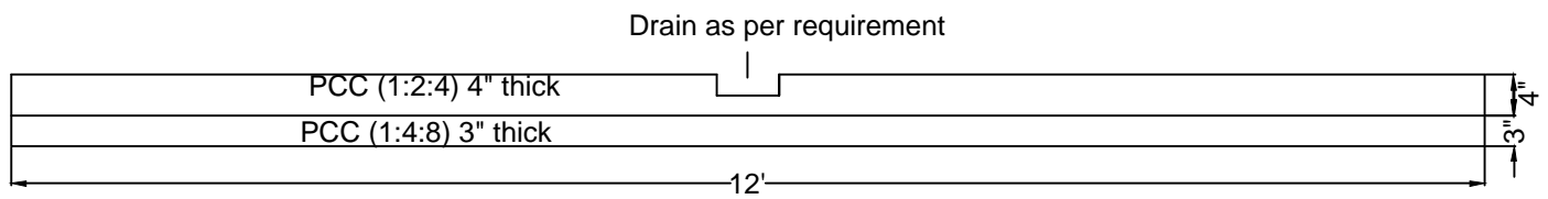
X-Section of Pavement of Steets at Alwargi and Hoti Kila
