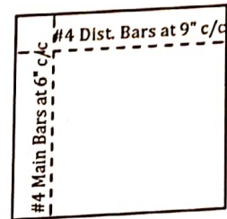
Room Roof Slab
