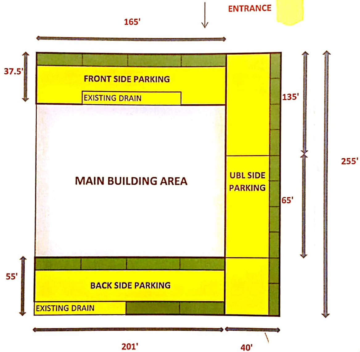
Drawing for Tuff Tile Installation for Parking Area of Main OGDCL Building
