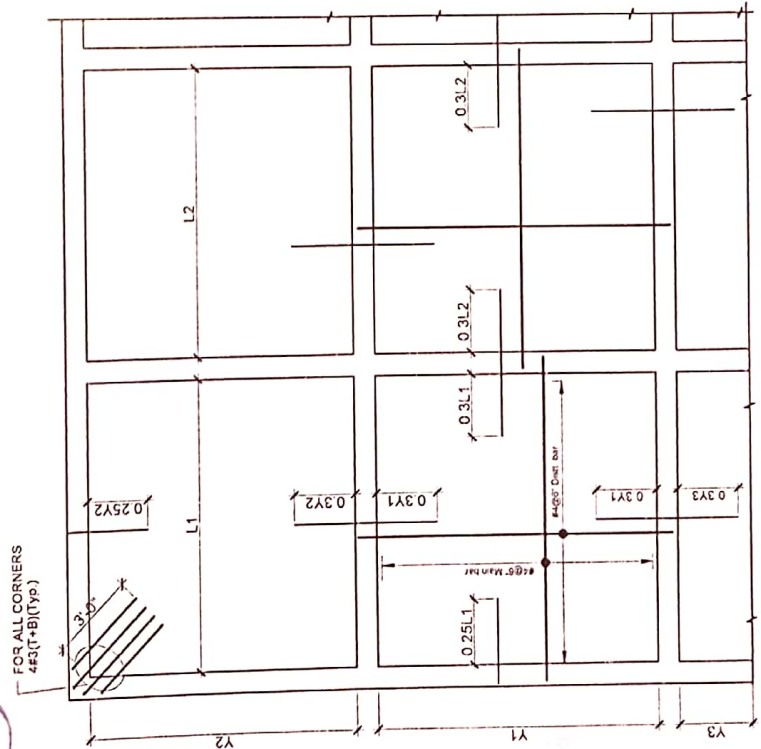
Typ. Plinth & Roof Beam Reinf. detail
