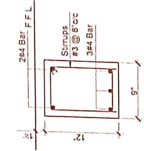
Plinth Beam PB-2
