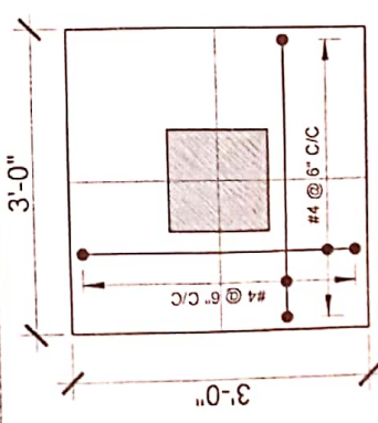
FOOTING (F1)
