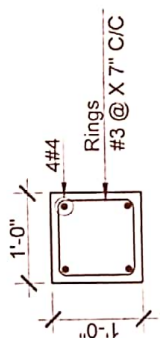
COLUMN (C1)
