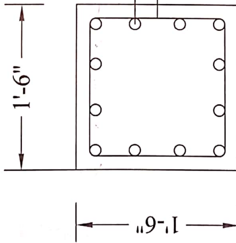
COLUMN (C1) STEEL REINFORCEMENT
