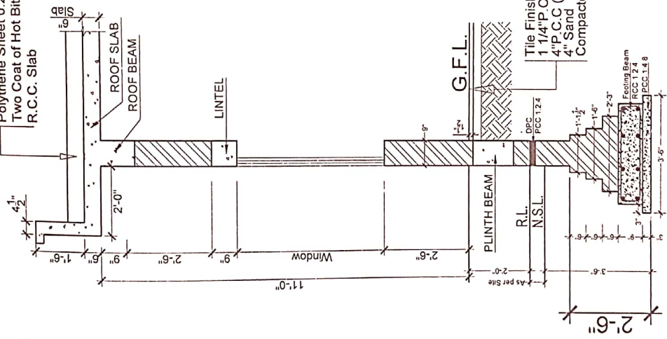
SECTION A-A (F1) FOOTING & COLUMN SECTION
