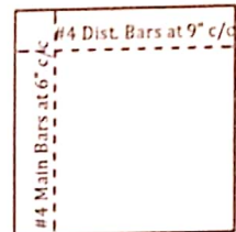
Room Roof Slab
