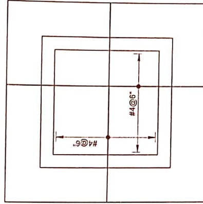
SLAB REINF. PLAN WATCH TOWER
