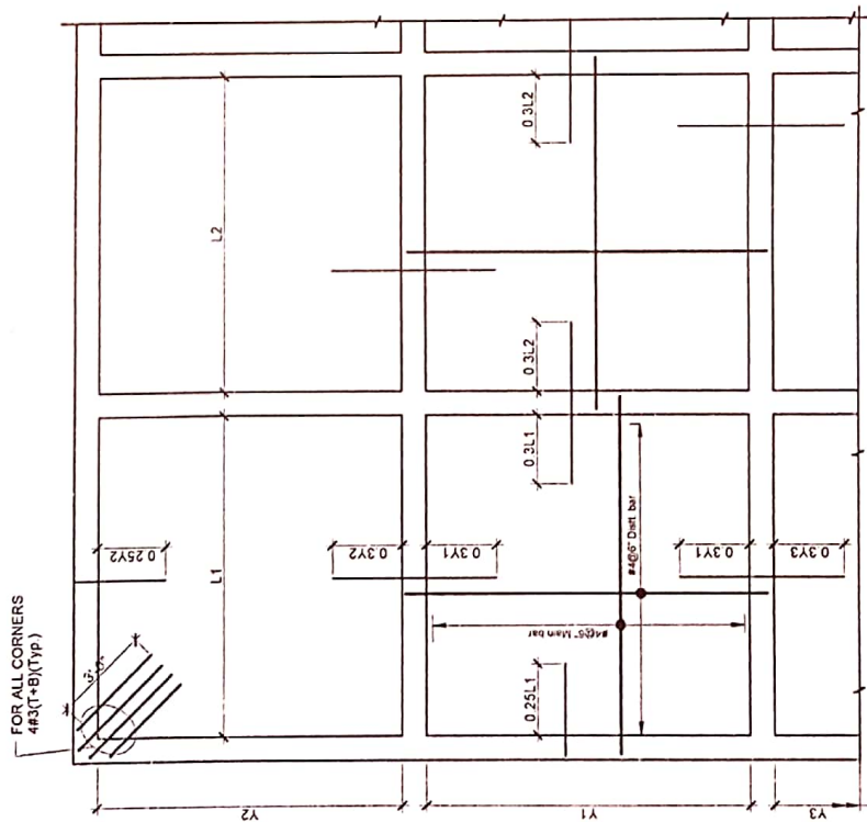
Typ. SLAB REINFORCEMENT (CUT OFF POINTS)
