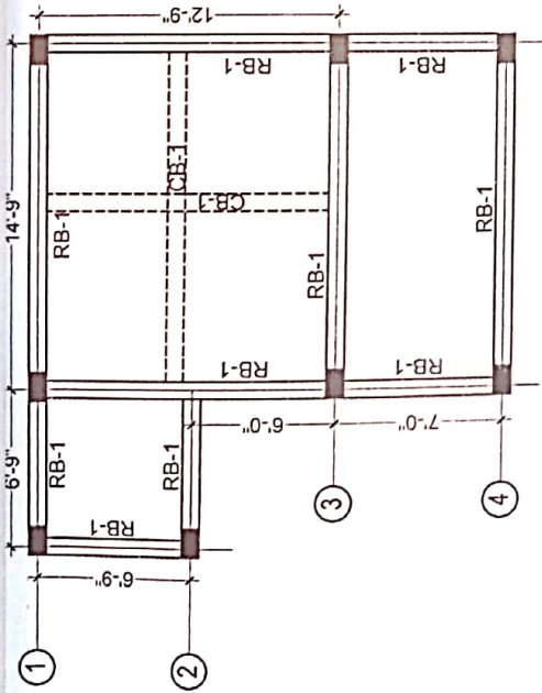
ROOF BEAM PLAN
