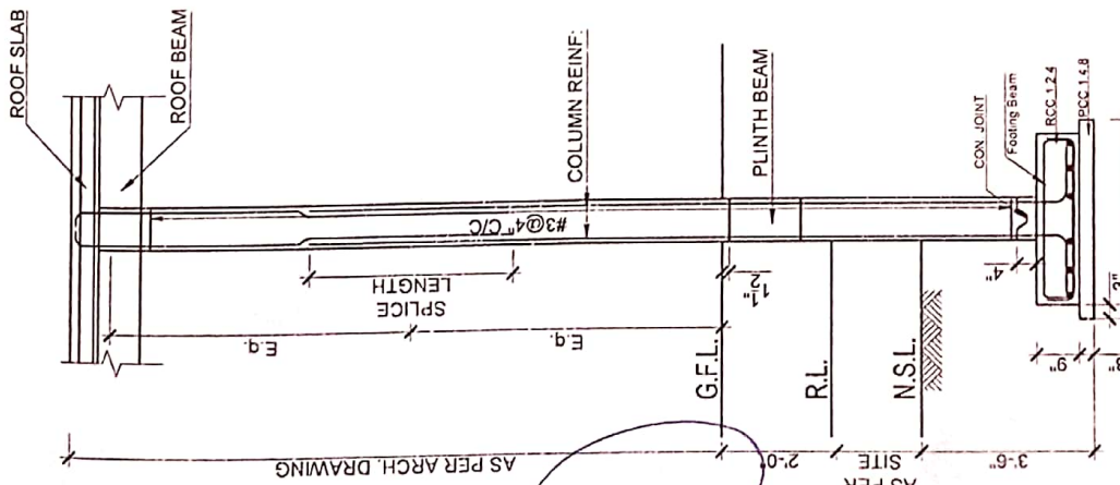
SECTION A-A (F1) FOOTING & COLUMN SECTION
