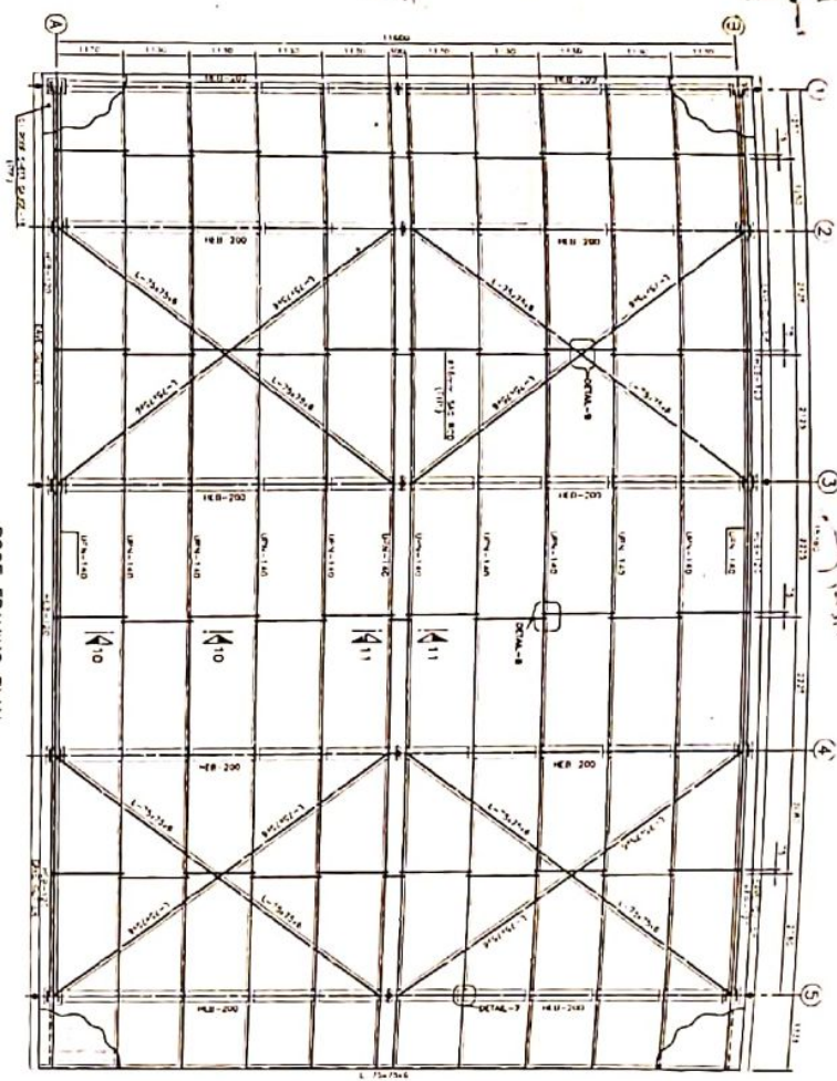
ROOF FRAMING PLAN SCALE: 1/25
