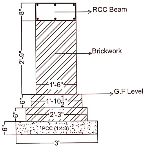
X-Section Crude Oil Tanks Foundation
