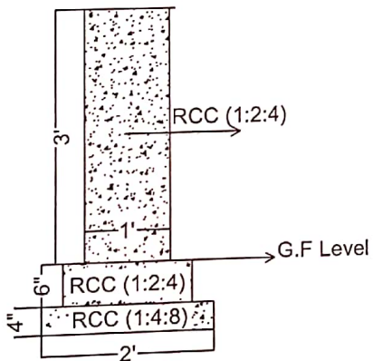
X-Section Pipe Sleepers Foundation
