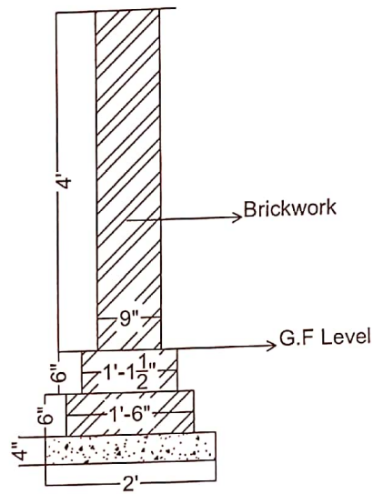
X-Section Dyke Wall Foundation
