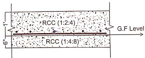
X-Section Separator Foundation
